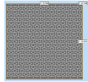
Relative Density – 50%
